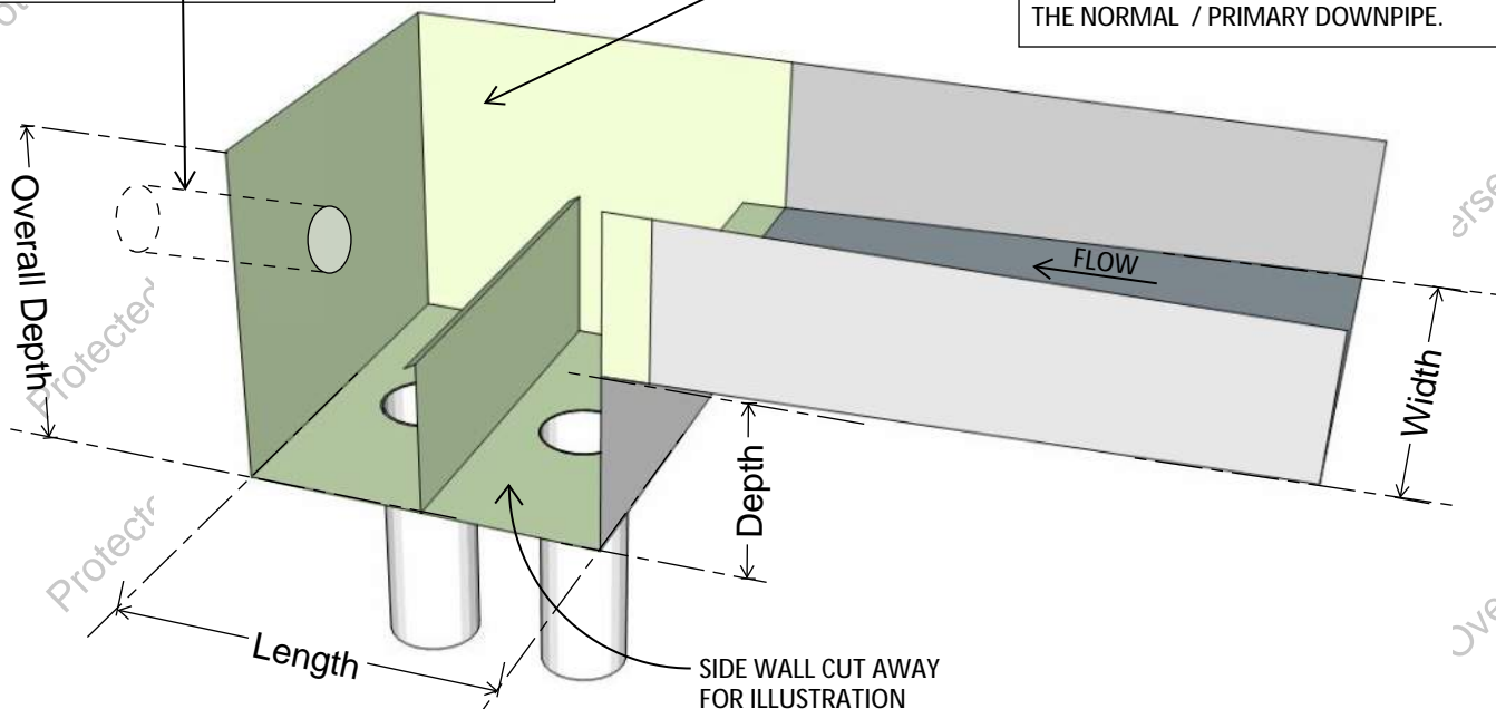
Sump dimensions
