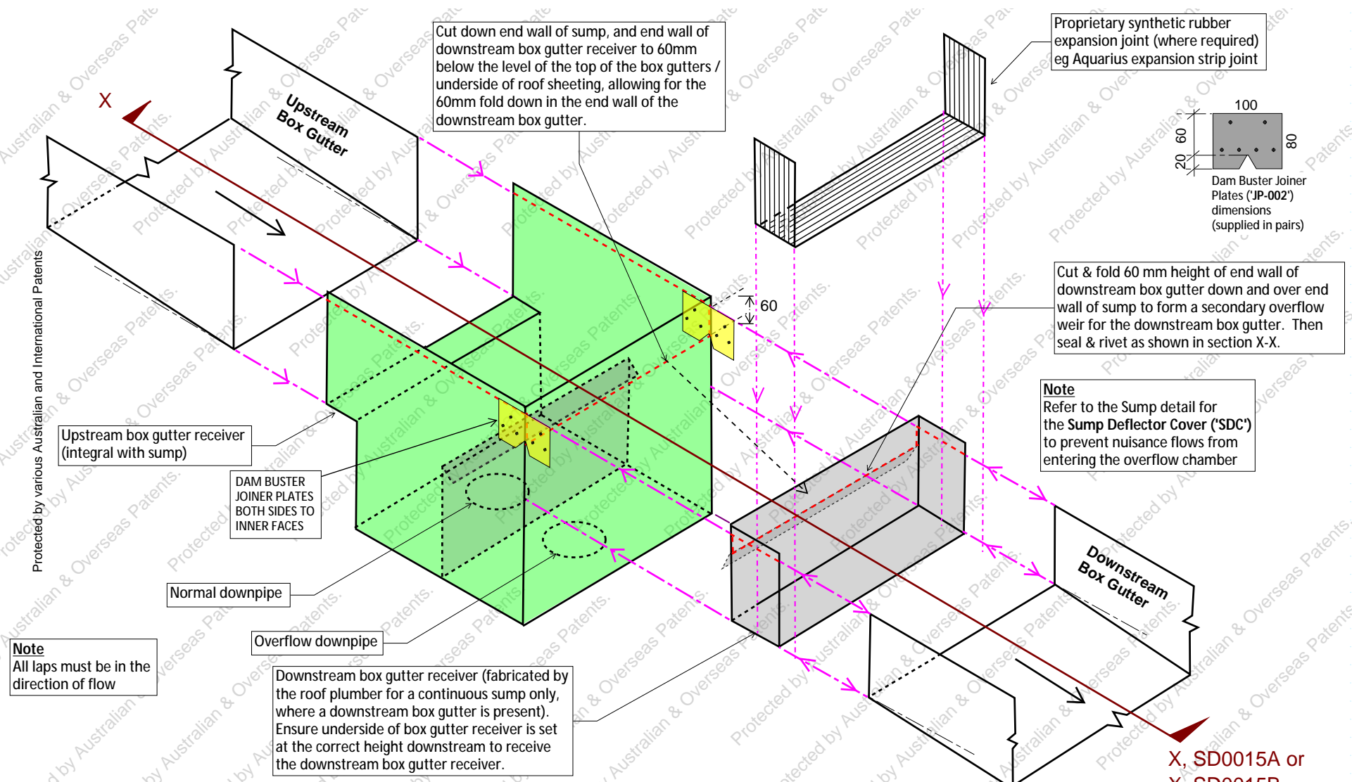
SD015 - Typical Dam Buster Continuous Sump with optional expansion joint detail (NTS)
